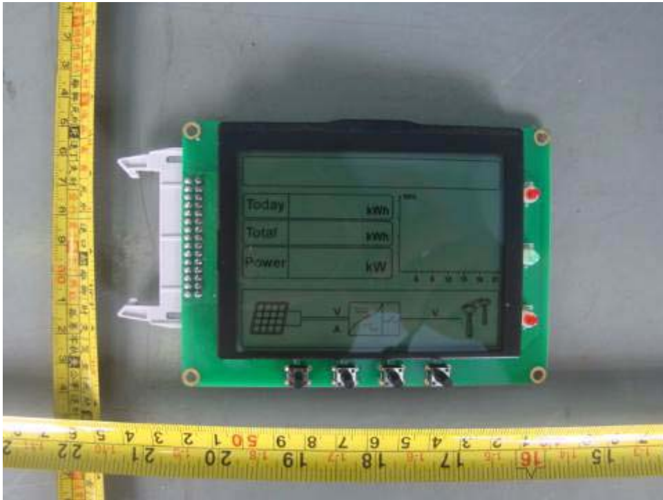
Component side of LCD board
